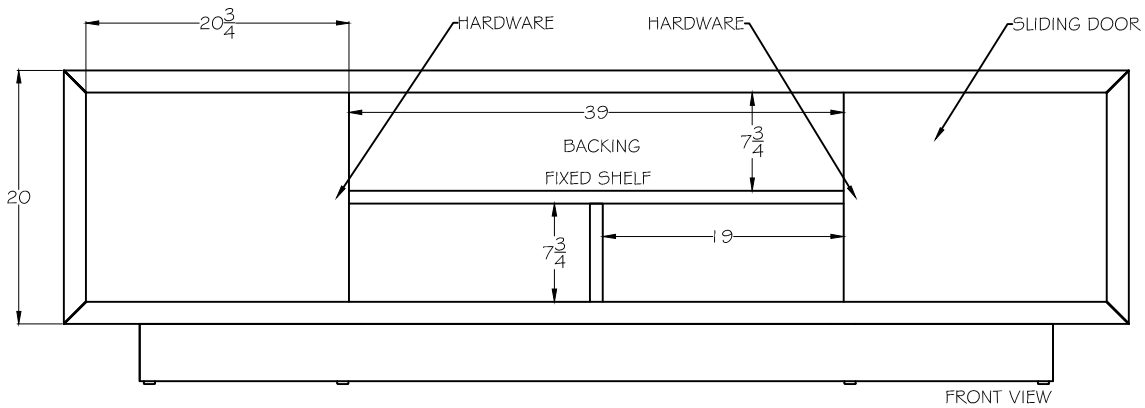
SLIDING DOORS AT ENDS POSITION
