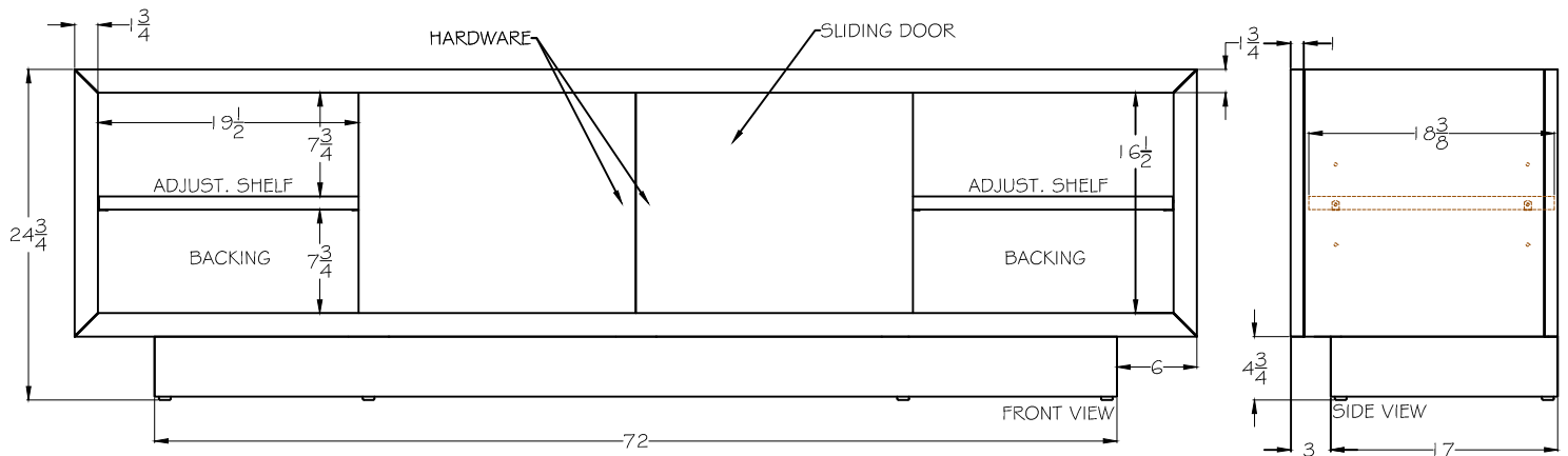
SLIDING DOORS AT CENTER POSITION
